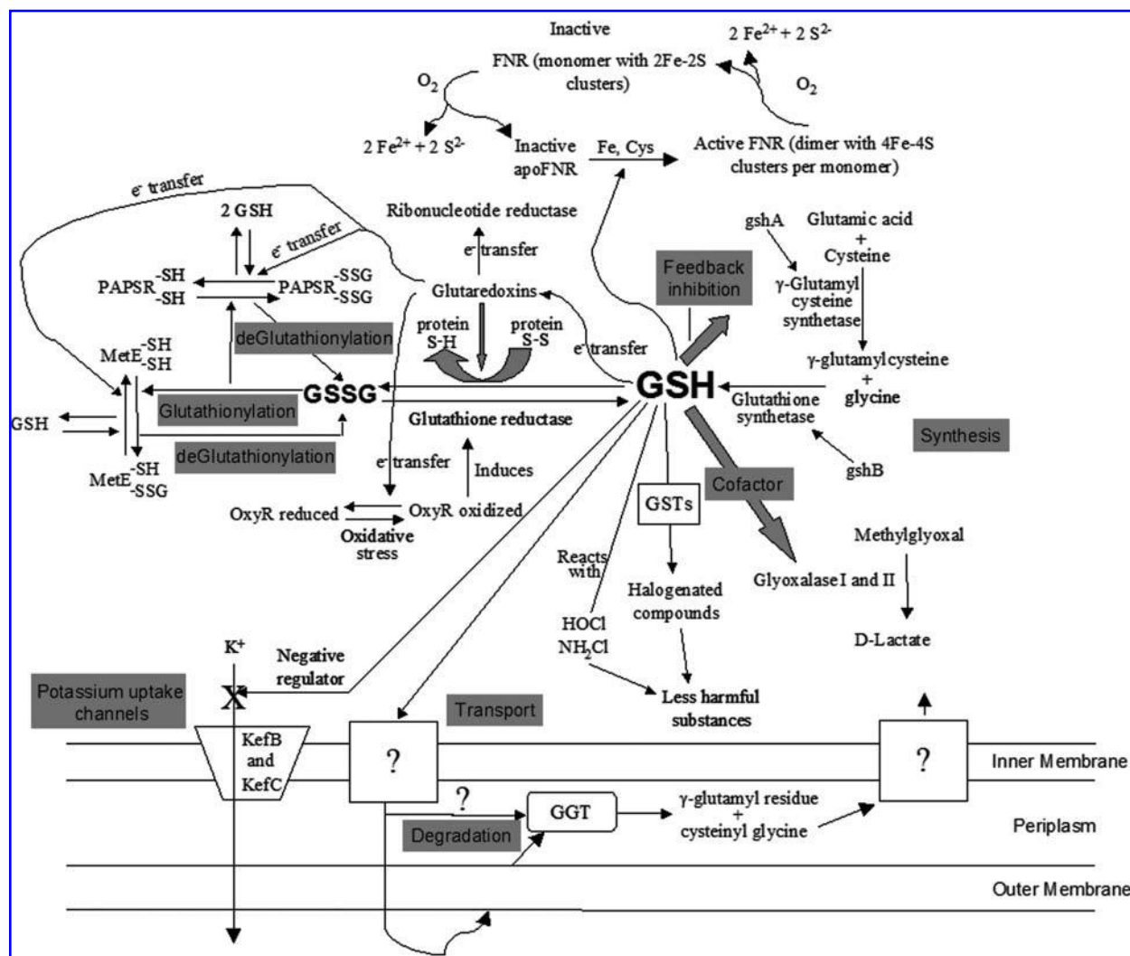
FIG. 1. The many faces of glutathione in E. coli .
