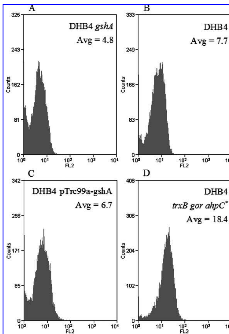
FIG. 3. Fluorescence distribution of E. coli in late exponential phase ( OD_{600} \approx 1 ) following labeling with the thiol specific probe mBBR. Histograms represent the mean fluorescence of 10000 E. coli events. (A) WP758 (DHB4 gshA ); (B) DHB4; (C) DHB4 pTrc99a- gshA ; (D) FA113 (DHB4 trxB gor ahpC* ). Flow cytometric assay conditions: Cells from single colonies were grown overnight in M9 casein media (1 X M9 minimal salts (Sigma, M6030), 0.4% (w/v) glucose, 0.1% (w/v) casein enzymatic hydrolysate (Sigma, C0626), 2 mM MgSO_4 , 0.05 mg/ml thiamine) with the appropriate antibiotic at 37°C with shaking. Cells were then subcultured 1:100 in fresh M9 casein media and grown to OD_{600} \approx 1 at which point 1 ml of cell culture was centrifuged (5 min at 10,000 RPM), the supernatant discarded and the pellet resuspended in 1 ml PBS. Cells were then incubated with monobromobimane (mBBR, Molecular Probes, M-1378) at a final concentration of 0.33 mM at room temperature for 60 min and analyzed for fluorescence emission with a flow cytometer (MoFLO, Cytomation). DHB4, WP758 and FA113 were obtained from Jon Beckwith's laboratory. Their genotype is as follows: DHB4 is MC1000 phoA (PvuII) phoR malF3 ; WP758 is DHB4 gshA ::Tn10Kan; FA113 is DHB4 gor522 . . . mini-Tn10Tc trxB ::Kan ahpC* .
